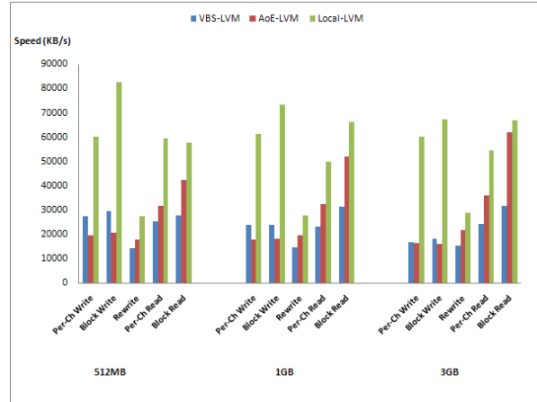
Figure 9 Performance comparison of VBS-LVM, AoE-LVM, and Local-LVM
